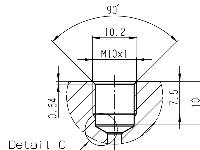
Installation recommendation Scale: 2:1
